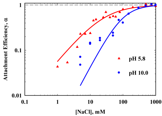
Figure 2. Effect of pH and IS on \alpha for O-MWCNTs treated with 15% \text{HNO}_3 at pH 5.8 \pm 0.2 and 10.0 \pm 0.2 .
